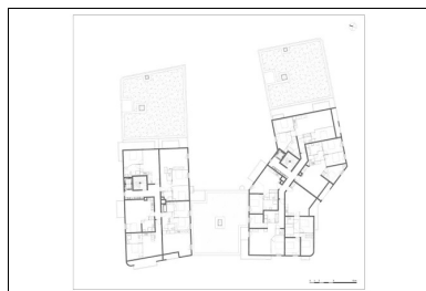
Plan R+5
